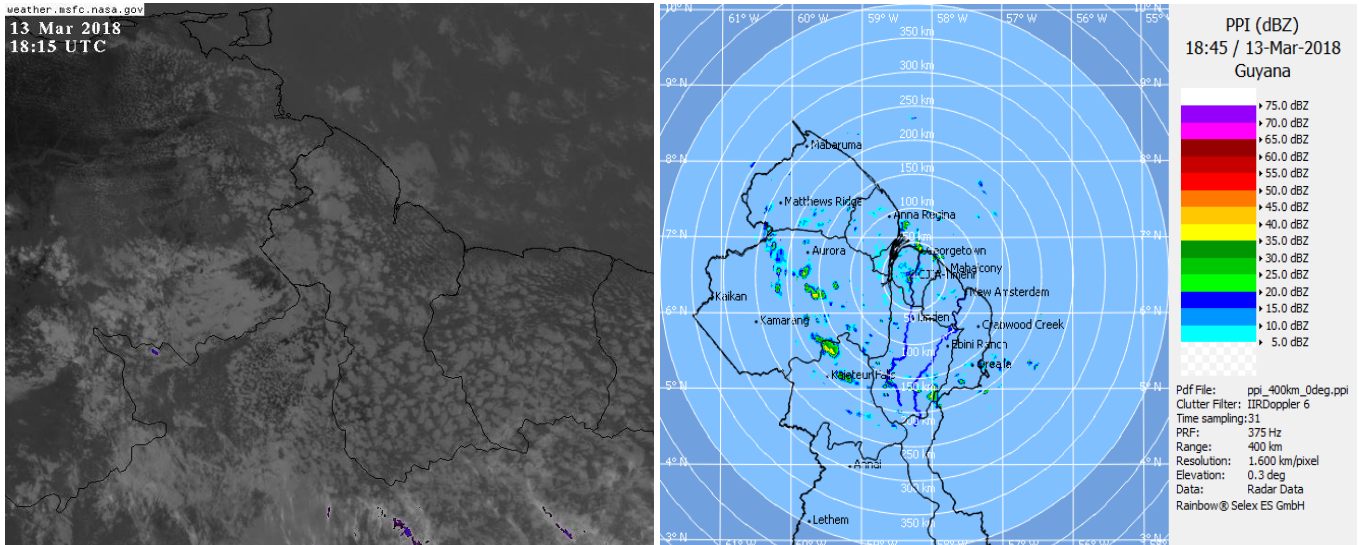
Infra-red Satellite image valid 18:15 UTC (14:15hrs) Tuesday March 13, 2018
