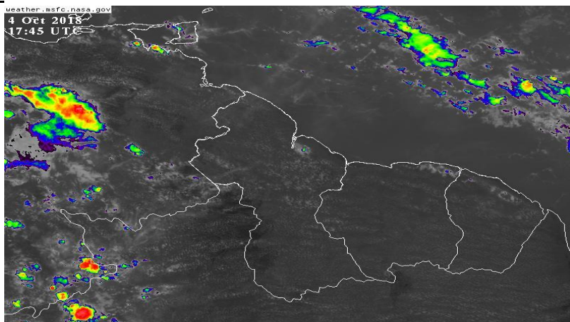
Infra-red Satellite valid 17:45 UTC (13:45hrs) Thursday October 04, 2018
