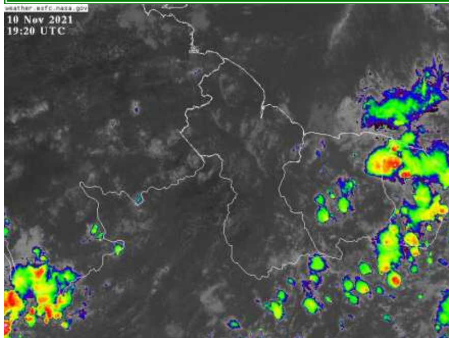
Satellite Imagery Valid 19:20 UTC/(15:20 LST) for Wednesday 10 November, 2021.
