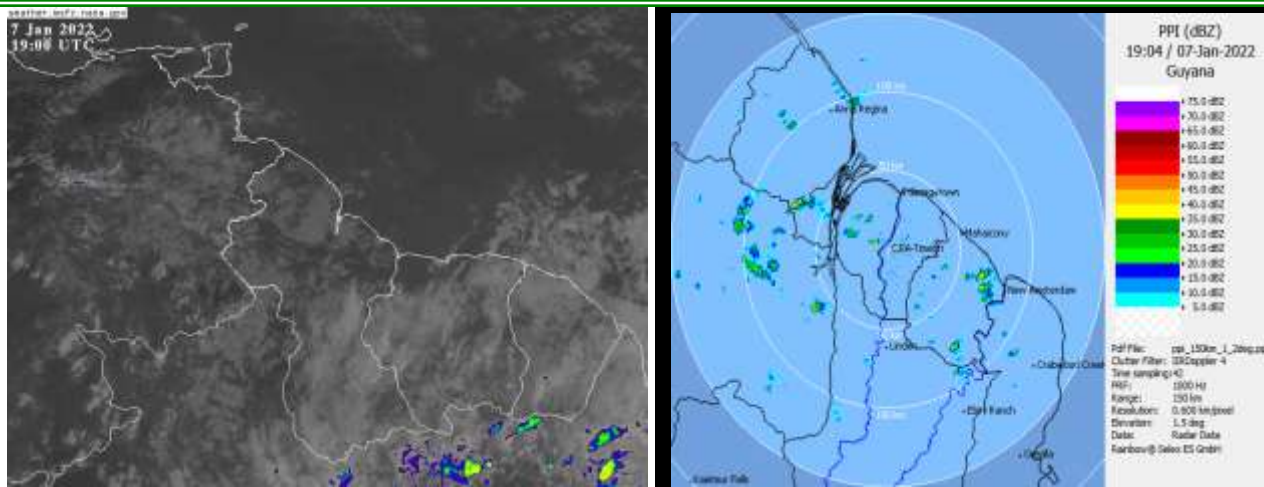
Satellite Imagery Valid 19:00 UTC/(15:00 LST) and Doppler Radar imagery Valid 19:04 UTC/ 15:04LST), Friday 07 January, 2022.
