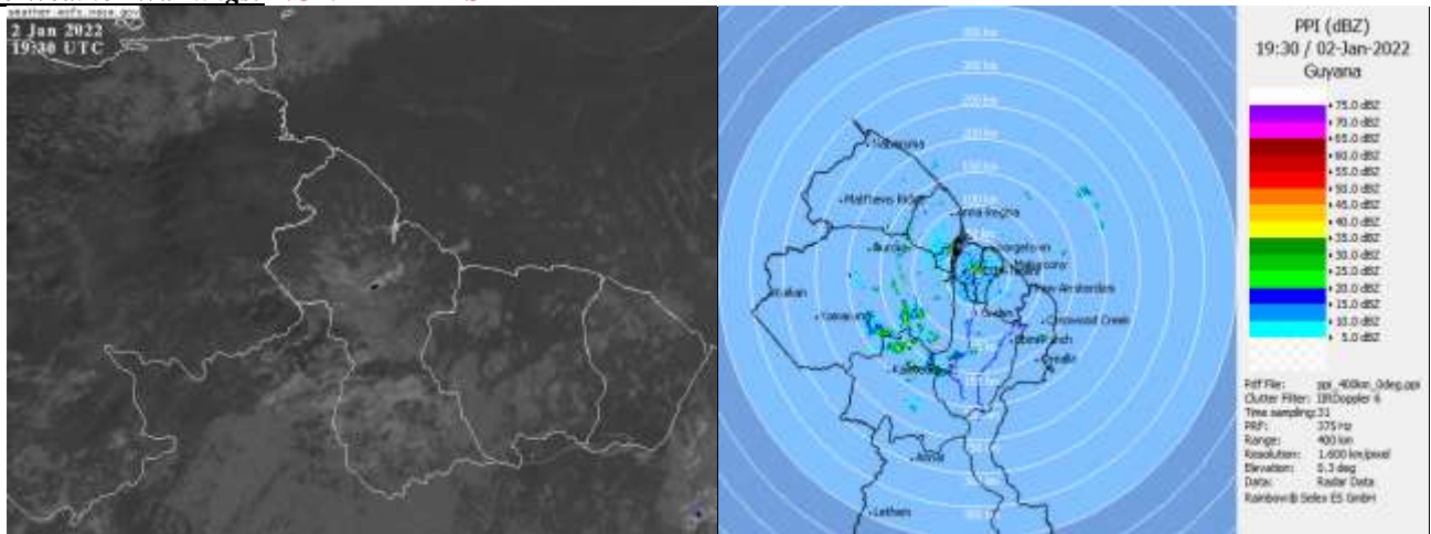
Infra-red Satellite and radar images valid 19:30 UTC (15:30hrs) Sunday January 02, 2022
