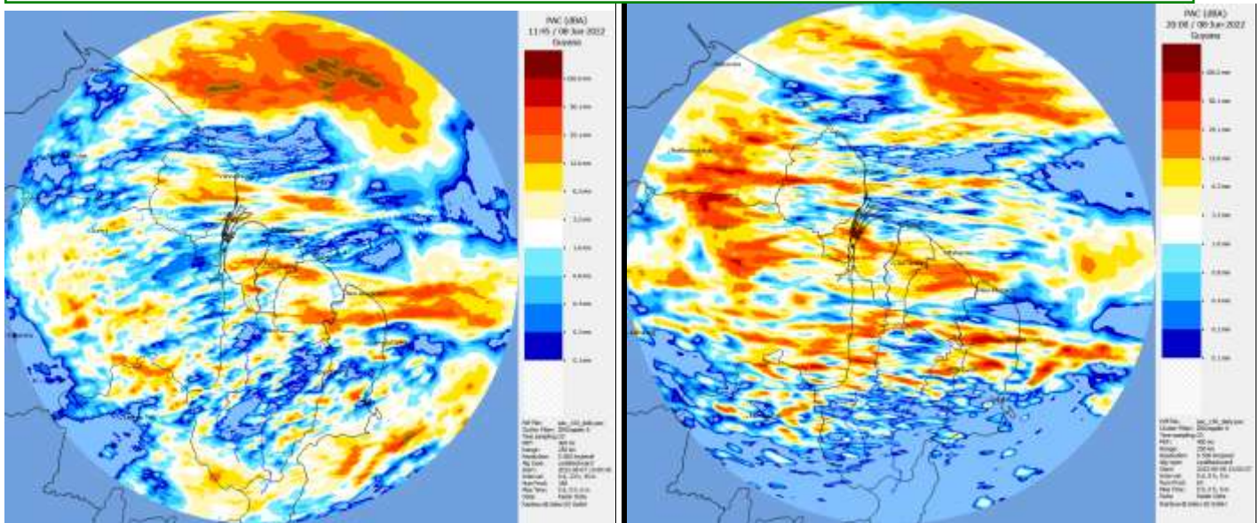
Radar generated precipitation estimates. Twenty-four and nine hours rainfall valid 7 hrs and 16 hrs, June 8, 2022.
