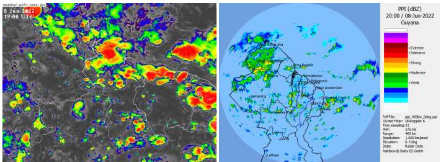
Infra-red Satellite and Radar images valid 18:10 UTC (14:10hrs) Wednesday June 8, 2022.
