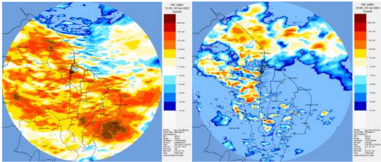
Radar generated precipitation estimates. Twenty-four and nine hours rainfall valid 8 hrs and 15 hrs, 03 June, 2022.
