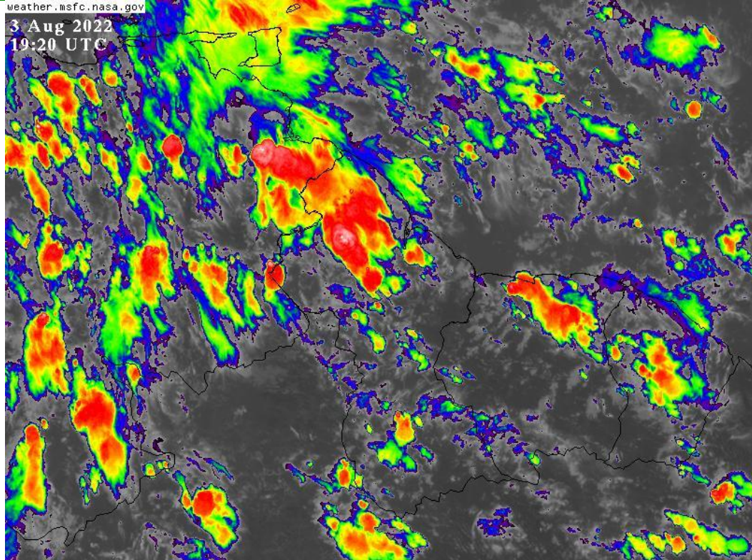
Satellite Imagery Valid 19:30 UTC/ (15:30 LST)
