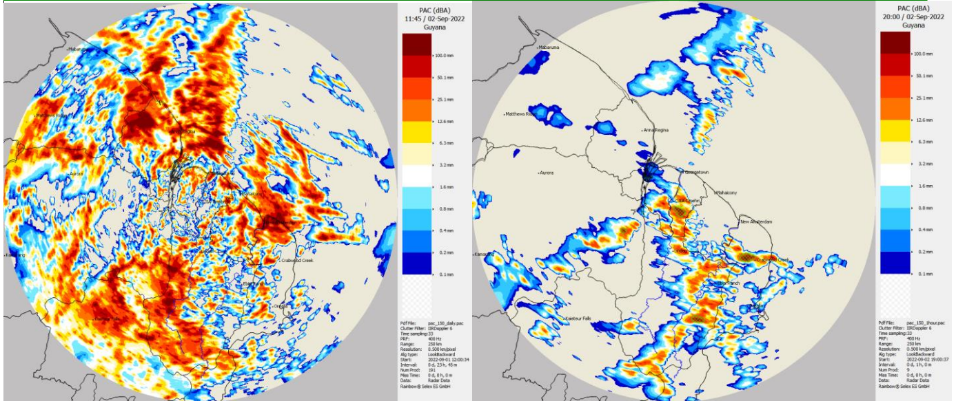
Radar generated precipitation estimates. Twenty-four- and nine-hours rainfall valid 7 hrs and 16 hrs, 02 September 2022.
