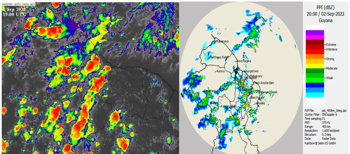
Infrared Satellite and Radar images valid 19:00 UTC (15:00hrs) Friday September 02, 2022.
