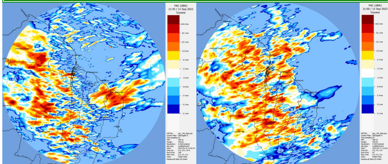
Radar generated precipitation estimates. Twenty-four and nine hours rainfall valid 7 hrs and 16 hrs, 11 September 2022. Table # 2 Occurrences of high and low tides for the next 24 hours and the times for sunrise and sun set.
