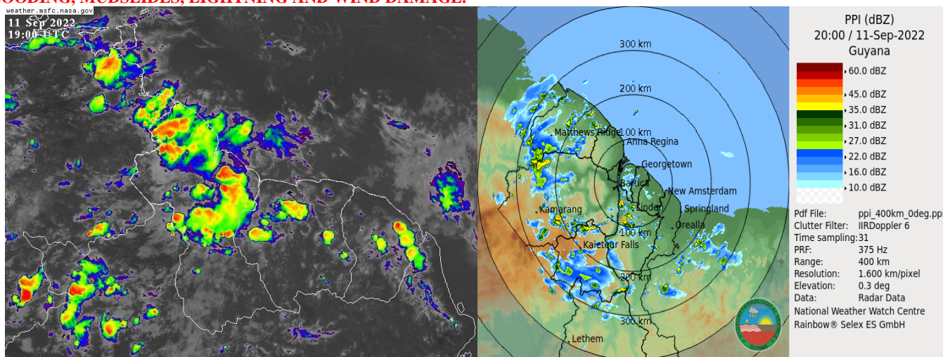
Infrared Satellite and Radar images valid 19:00 UTC (15:00hrs) Sunday September 11, 2022.
