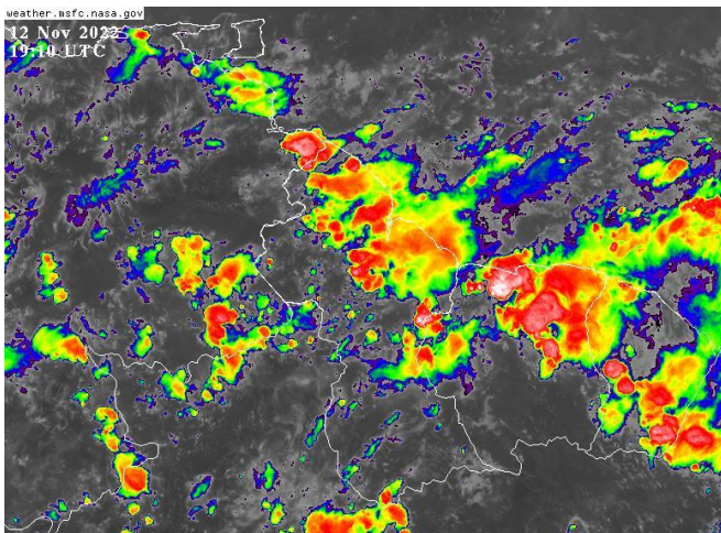
Infrared Satellite and Radar images valid 19:10 UTC (15:10 hrs) Saturday November 12, 2022.
