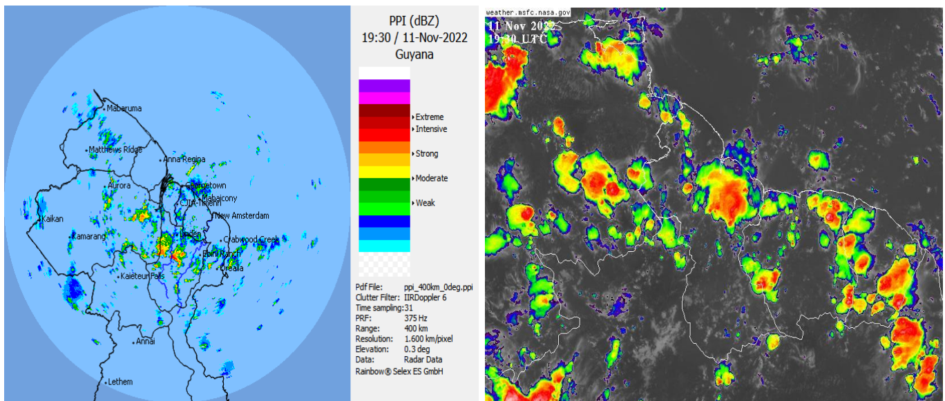
Infrared Satellite and Radar images valid 19:30 UTC (15:30hrs) Friday November 11, 2022.
