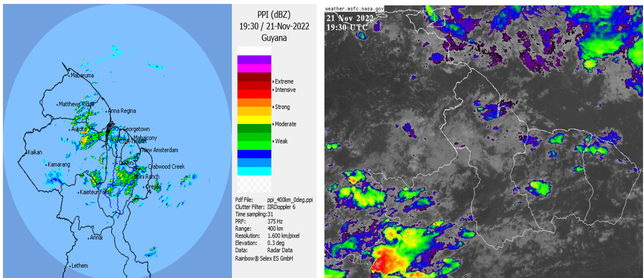
Infrared Satellite and Radar images valid 19:30 UTC (15:30hrs) Monday November 21, 2022.
