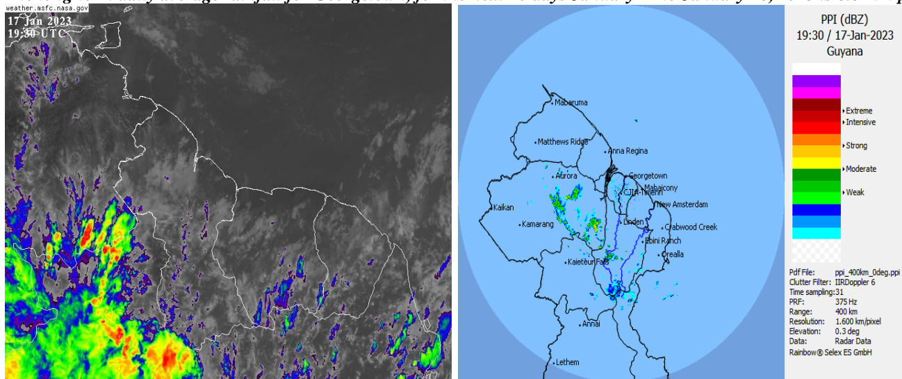
Infrared Satellite & Radar images valid 19:30 UTC (15:30hrs) Tuesday January 17, 2023.
