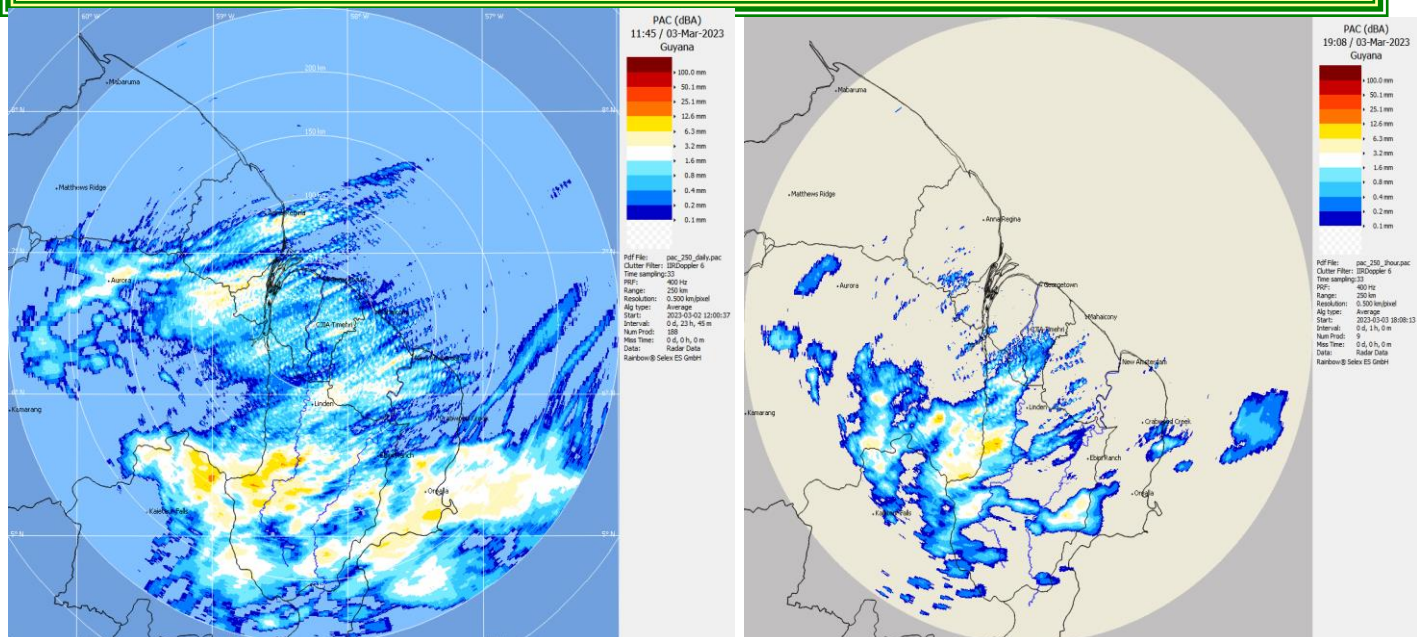
Radar generated precipitation estimates. Twenty-four- and nine-hours rainfall valid 7 hrs and 16 hrs, 03 March, 2023.
