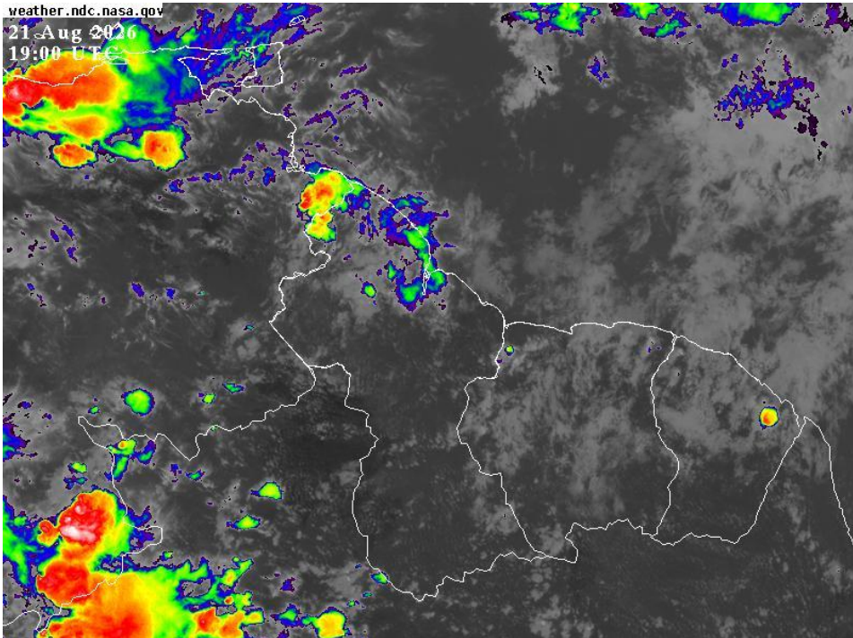
Infrared Satellite image valid 19:00 UTC (15:00 hrs) Friday, 21 August 2026
