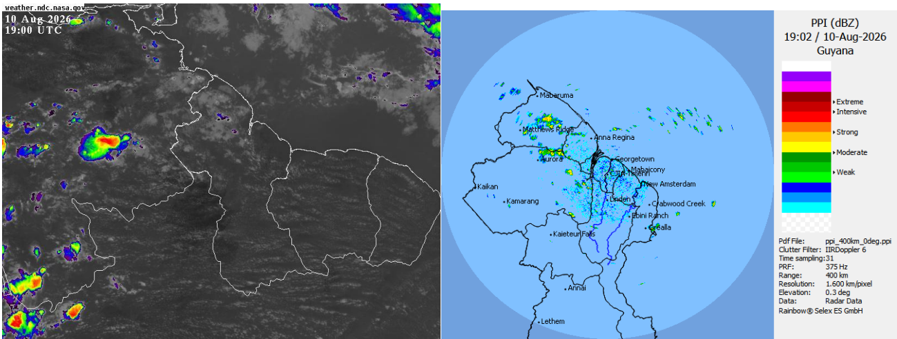
RADAR and Infrared Satellite images valid at 19:00 UTC (15:00 hrs)
