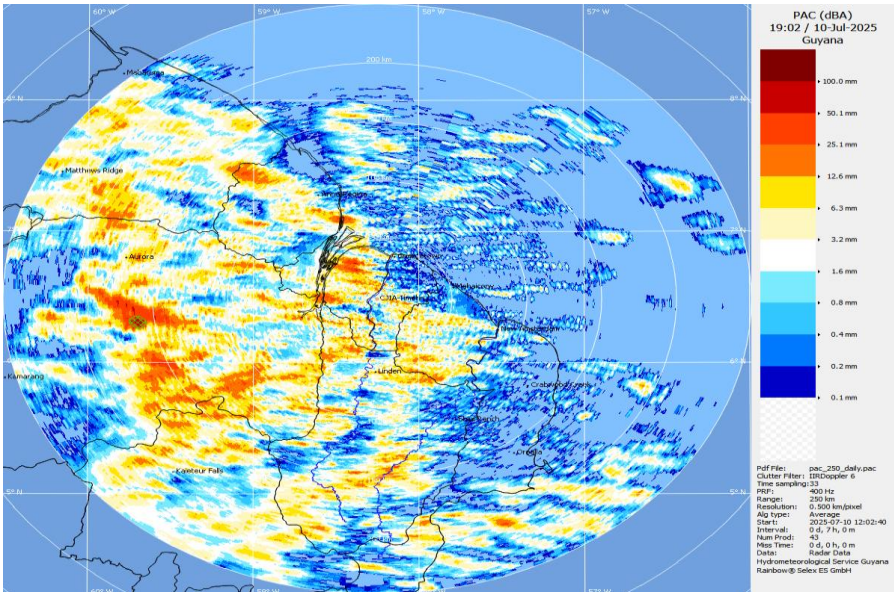
Seven(7) hours Precipitation Accumulation image (PAC) from 12:02 UTC (08:02 hrs) to 19:02 UTC (15:02 hrs).
