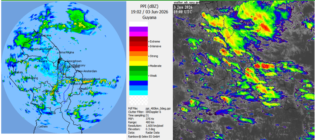
RADAR and Infrared Satellite images valid at 19:00 UTC (15:00 hrs)
