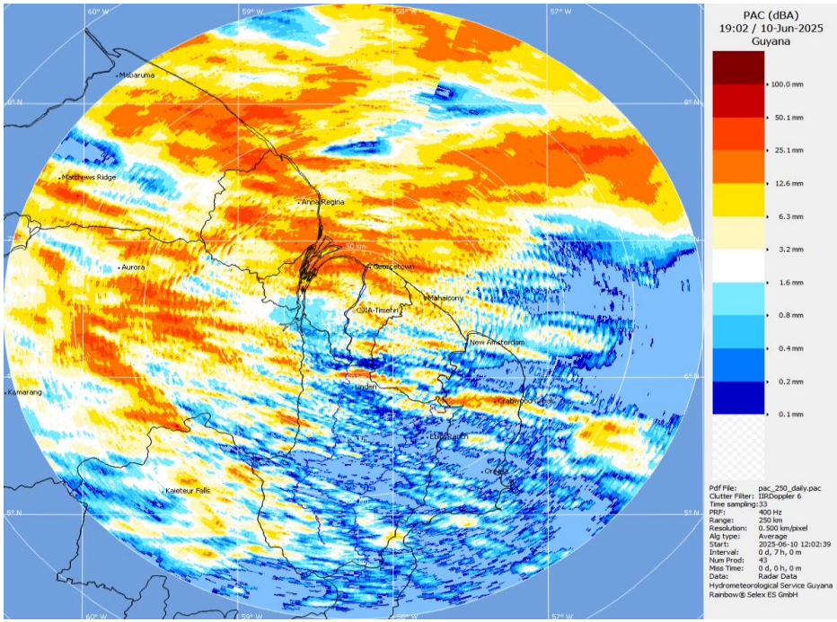
Seven(7) hours Precipitation Accumulation image (PAC) from 12:02 UTC (08:02 hrs) to 19:02 UTC (15:02 hrs)
