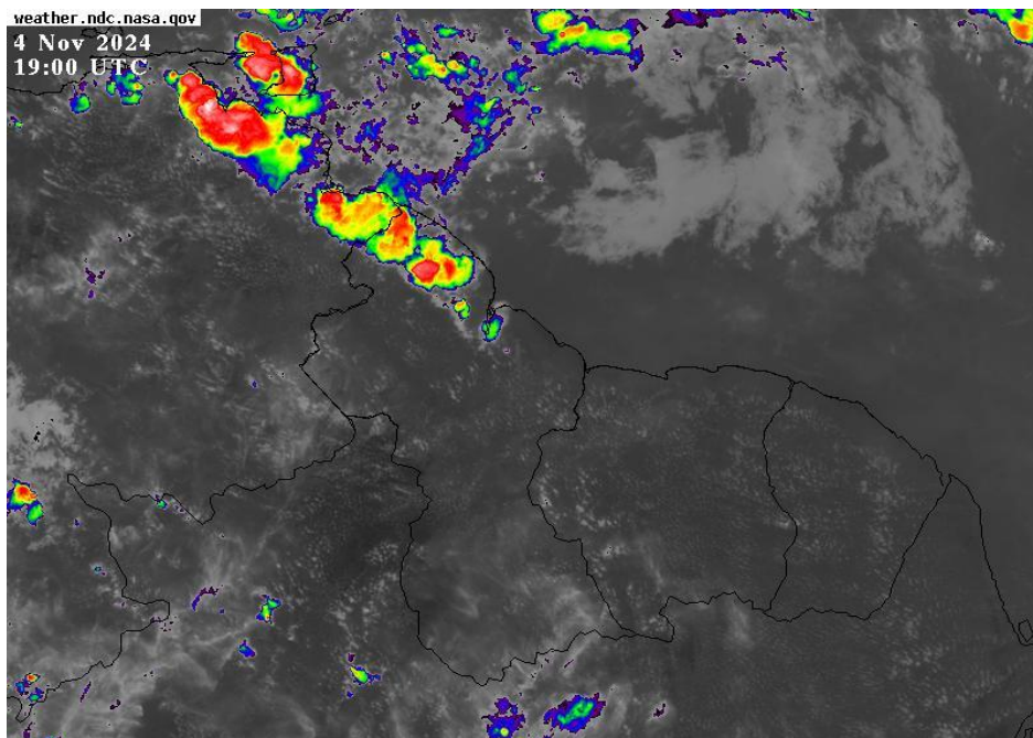
Infrared Satellite image valid at 19:00 UTC (15:00 hrs)
