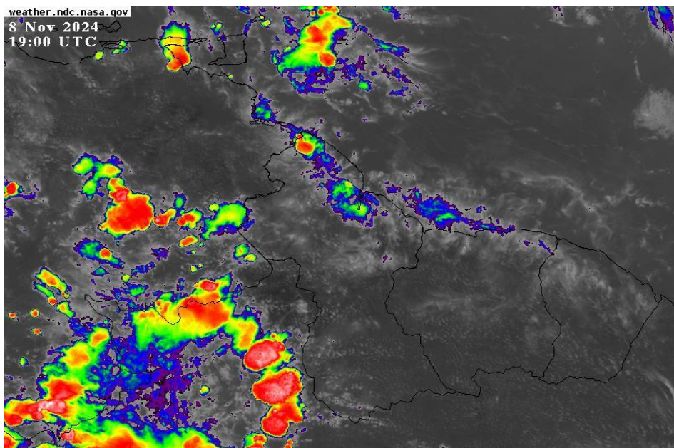
Infrared Satellite image valid at 19:00 UTC (15:00 hrs)
