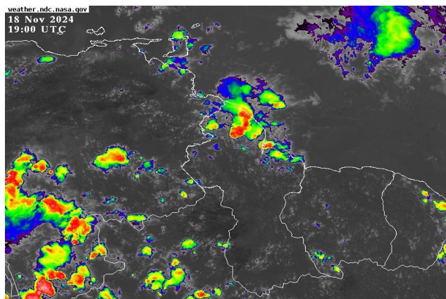
Infrared Satellite image valid at 19:00 UTC (15:00 hrs)
