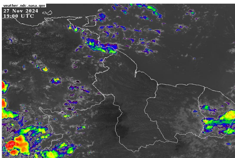
Infrared Satellite image valid at 19:00 UTC (15:00 hrs)
