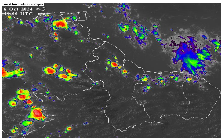
Infrared Satellite image valid at 19:00 UTC (15:00 hrs) Tuesday, October 8, 2024.
