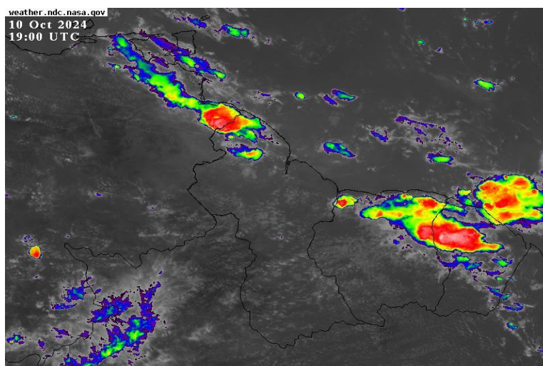
Infrared Satellite image valid at 19:00 UTC (15:00 hrs) Thursday, October 10, 2024.
