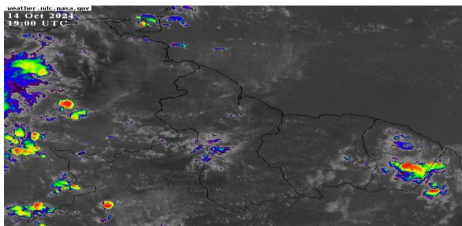
Infrared Satellite image valid at 19:00 UTC (15:00 hrs) Monday, October 14, 2024.
