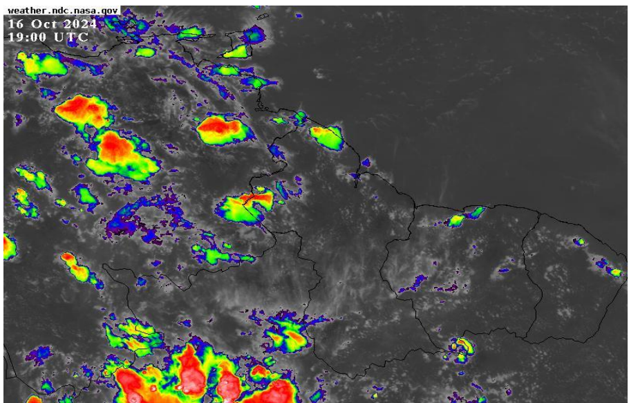
Infrared Satellite image valid at 19:00 UTC (15:00 hrs) Wednesday, October 16, 2024.
