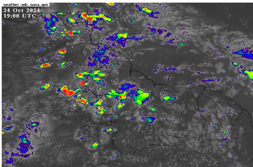
Infrared Satellite image valid at 19:00 UTC (15:00 hrs) Thursday, October 24, 2024.
