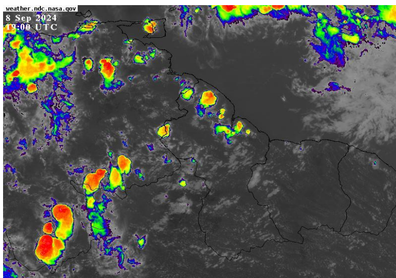
Infrared Satellite image valid at 19:00 UTC (15:00 hrs) Sunday, September 8, 2024.
