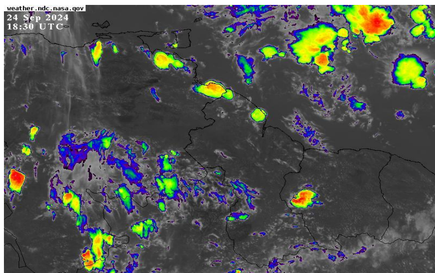
Infrared Satellite image valid at 18:30 UTC (14:30 hrs) Tuesday, September 24, 2024.
