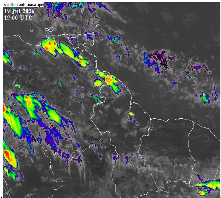
The Infrared Satellite image is valid at 19:00 UTC (15:00hrs) on Sunday, 19 July 2026.
