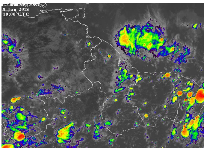
The Infrared Satellite image is valid at 19:00 UTC (15:00hrs) on Tuesday, 09 June 2026.
