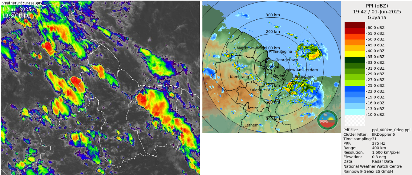
Infrared Satellite and Radar images valid 19:30 UTC (15:30hrs) Sunday, 01 June 2025
