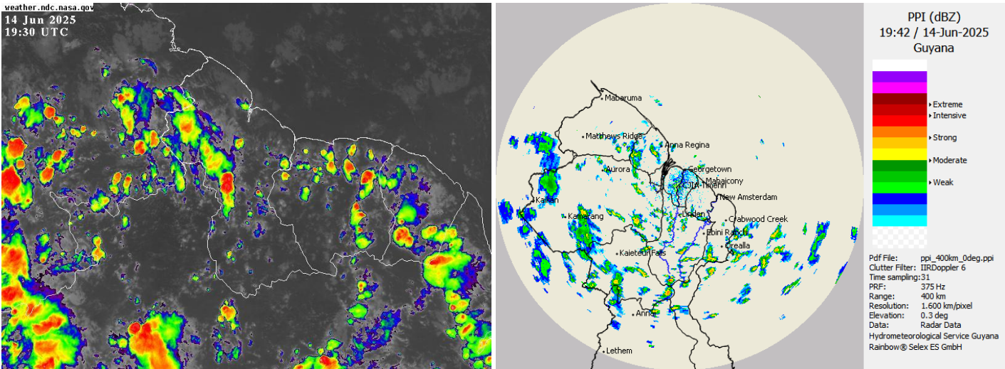
Infrared Satellite and Radar images valid 19:30 UTC (15:30hrs) Saturday, 14 June 2025
