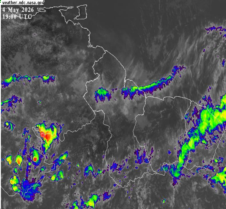
The Infrared Satellite image is valid at 19:00 UTC (15:00hrs) on Monday, 04 Mayl 2026.
