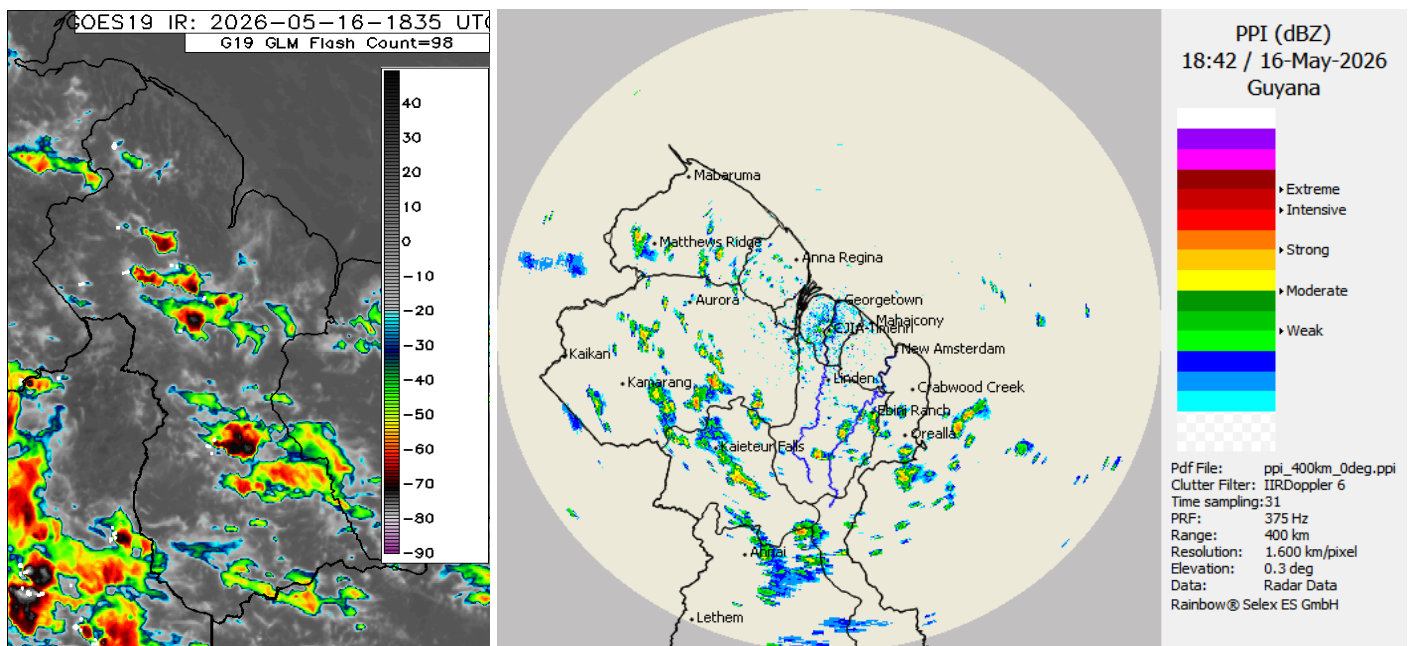
Infrared Satellite and Radar images valid 14:35 UTC (14:35 hrs) Saturday, 16 May 2026
