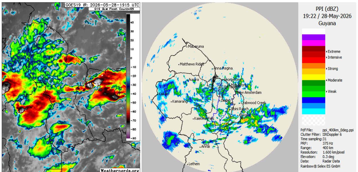
Infrared Satellite and Radar images valid 19:20 UTC (15:20 hrs) Thursday, 28 May 2026
