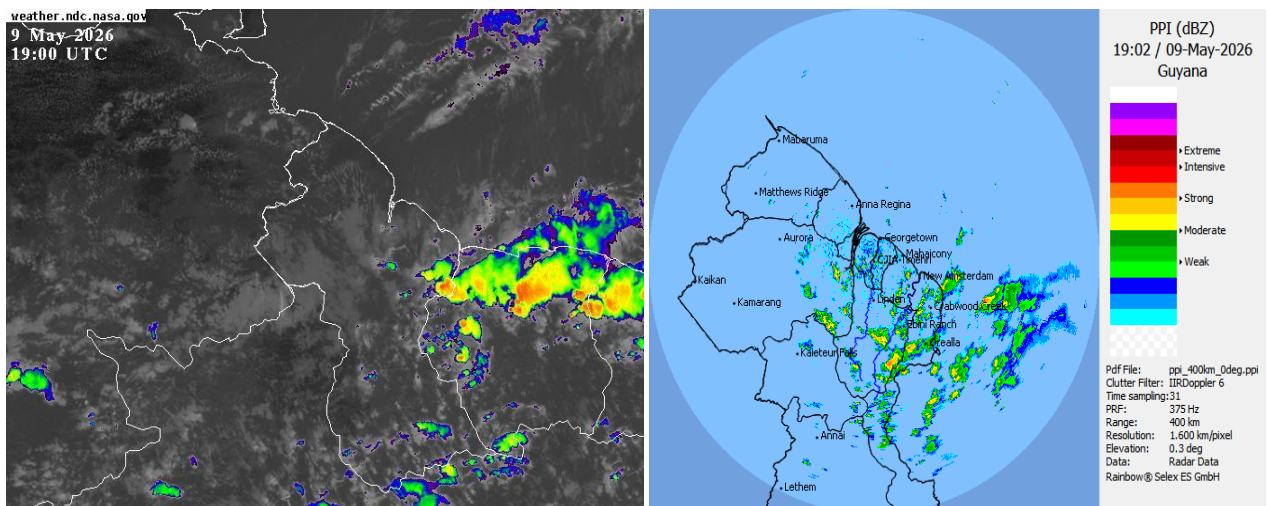
Infrared Satellite and Radar images valid 19:00 UTC (15:00 hrs) Saturday, 09 May 2026
