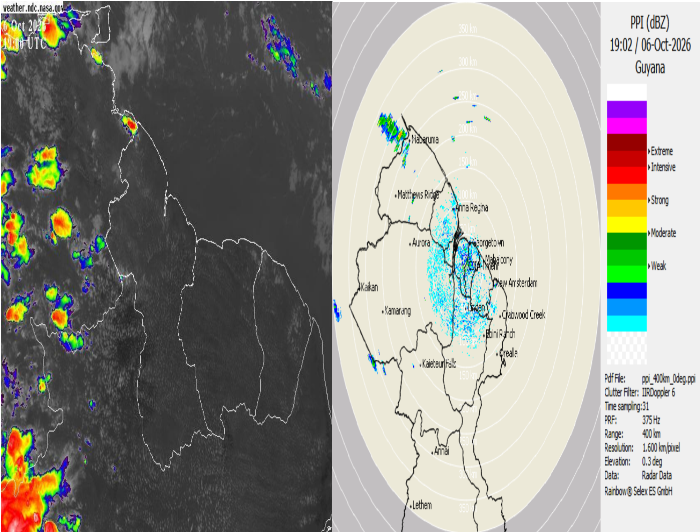
Infrared Satellite image valid 19:00 UTC (15:00hrs) 06/10/26.
