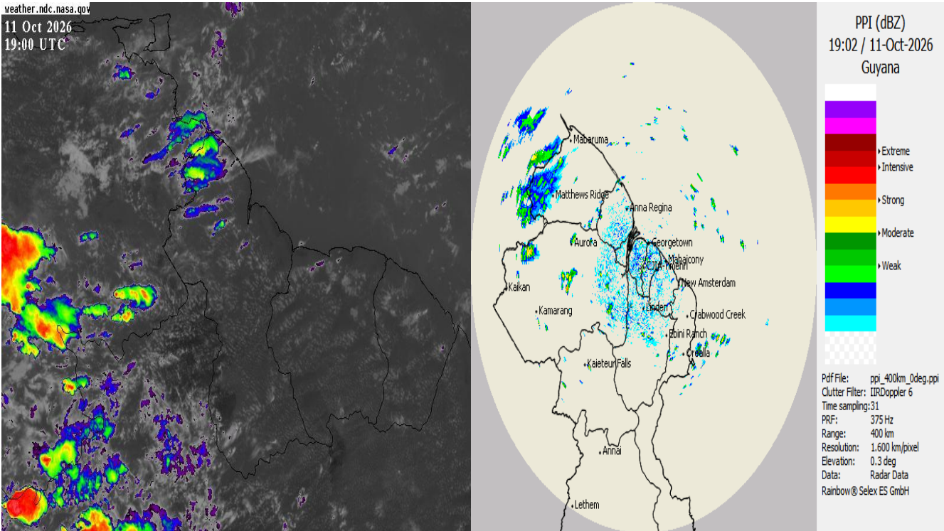
Infrared Satellite image valid 19:00 UTC (15:00hrs) 11/10/26.
