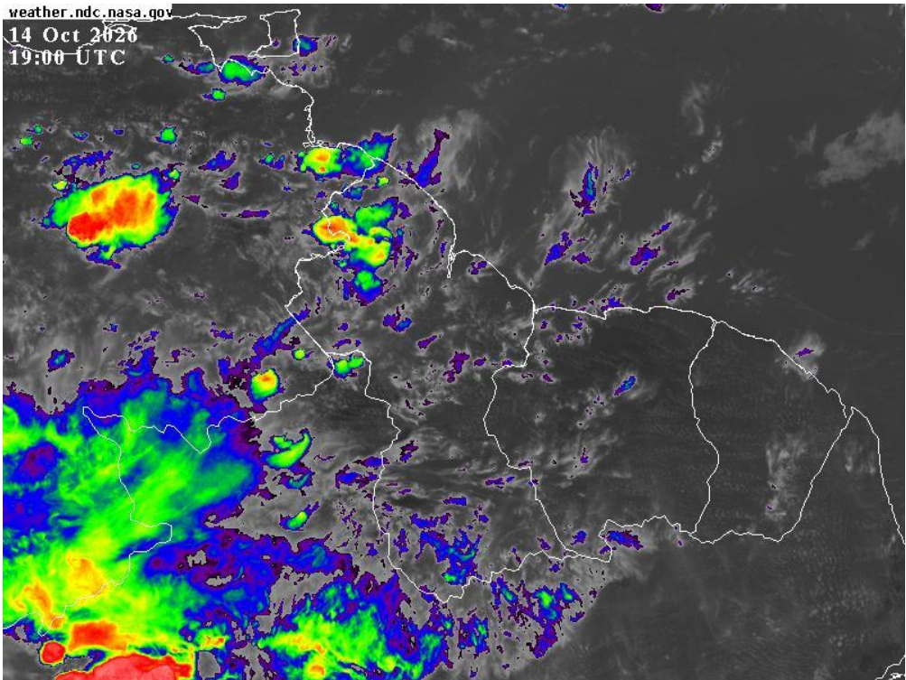
Infrared Satellite image valid at 19:00 UTC (15:00 hrs) Wednesday, 14 October 2026
