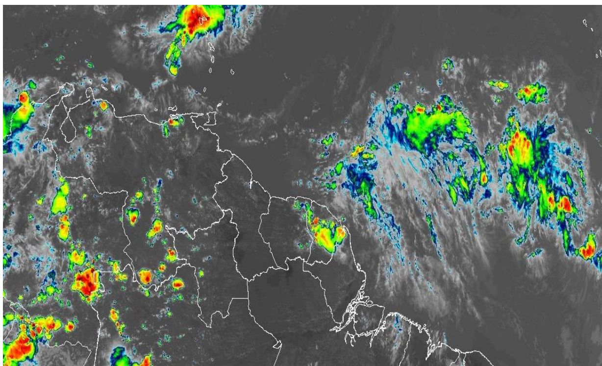
16 Oct 2025 19:00Z - NOAA/NESDIS/STAR - GOES-19 - Band 13 - TAW
