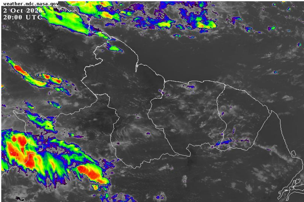
Infrared Satellite image valid at 20:00 UTC (16:00 hrs) Friday, 02 October 2026
