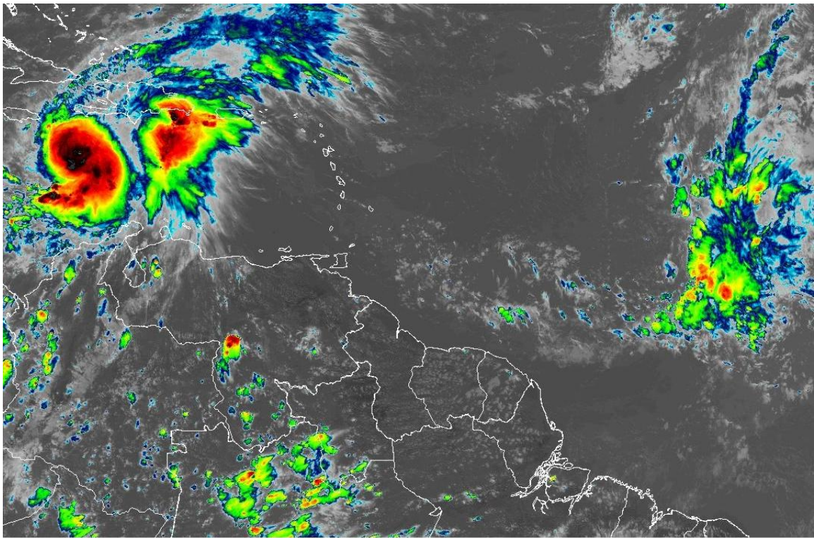
24 Oct 2025 19:00Z - NOAA/NESDIS/STAR - GOES-19 - Band 13 - TAW
