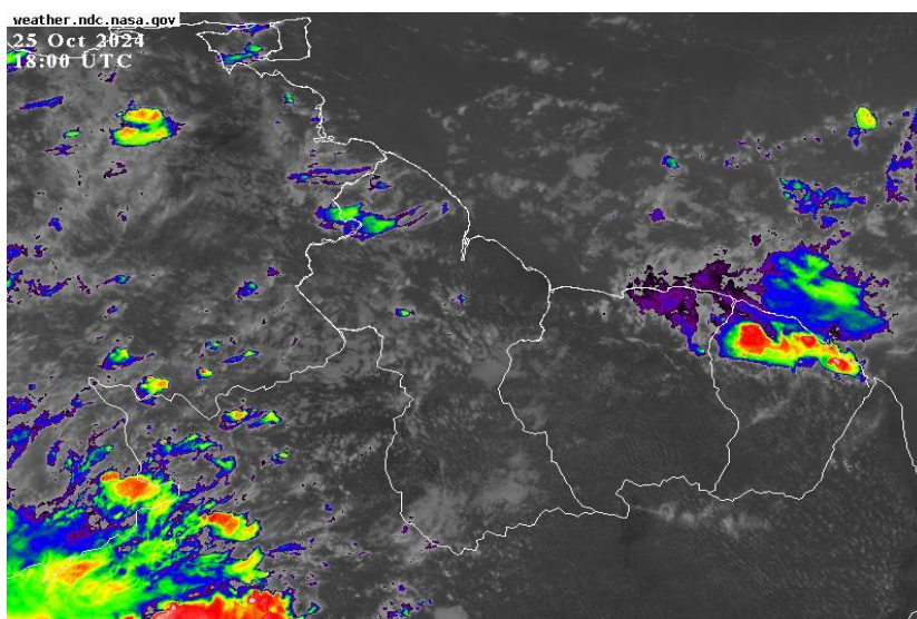
Infrared Satellite image valid 18:00 UTC (14:00hrs) Friday, 25 October 2024.
