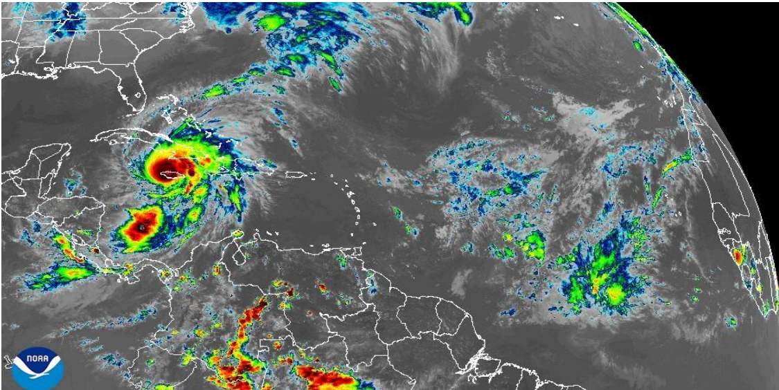
28 Oct 2025 19:40Z - NOAA/NESDIS/STAR - GOES-19 - Band 14 Infrared Satellite images valid 19:40 UTC (15:40 hrs) Tuesday, 28 October 2025
