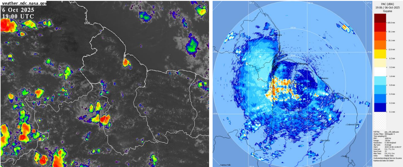
Infrared Satellite Radar-generated precipitation estimates images valid 19:00 UTC (15:00 hrs) Monday, 06 October 2025
