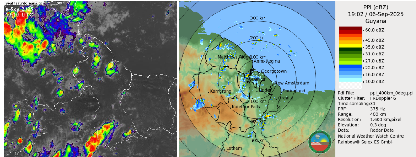
Infrared Satellite and Radar images valid 19:10 UTC (15:10 hrs) Saturday, 06 September 2025
