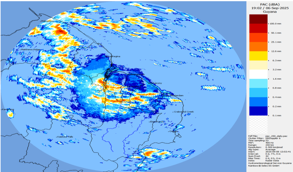
Radar-generated precipitation estimates at 15 hrs for seven hours of rainfall, Saturday, 06 September 2025.
