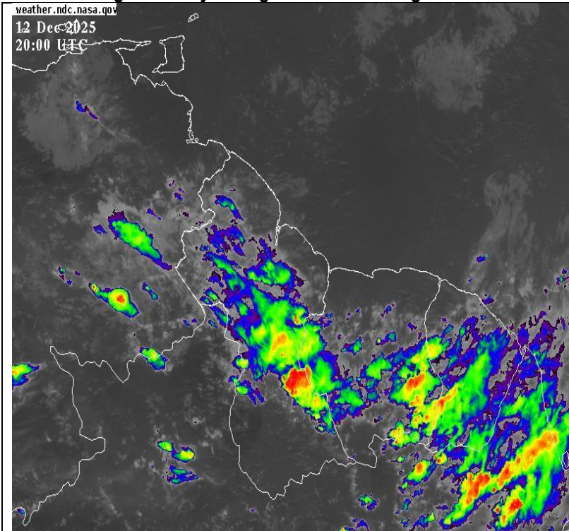
Infrared Satellite image valid at 16:00 UTC (16:00hrs) Friday, 12 December 2025.
