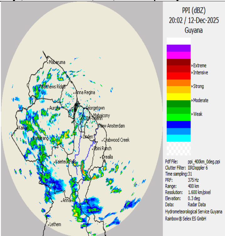
Radar image valid at 16:02 UTC (16:02hrs) Friday, 12 December 2025.
